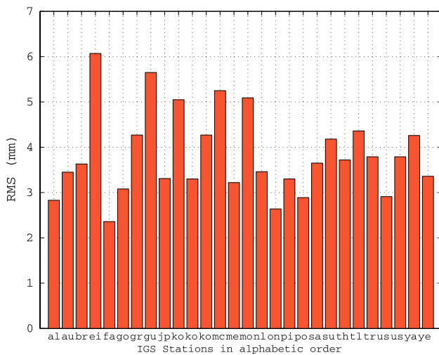
Fig. 4 The RMS of ZPD differences between the new and legacy strategies for each site selected for the comparison. x -axis denotes the station list in alphabetic order; y -axis denotes the RMS of the ZPD differences in mm
