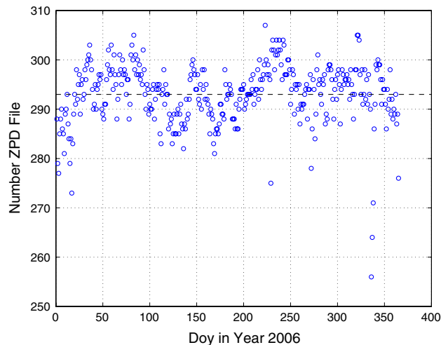
Fig. 5 The number of IGS troposphere ZPD files for each day in year 2006
