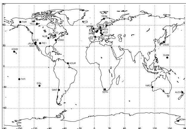
Fig. 1 The subset of global IGS stations used for comparing the new and legacy ZPD
