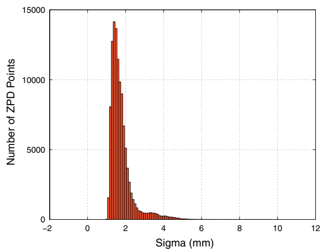
Fig. 3 Histogram of the formal errors reported for the new Final troposphere product. The histogram was generated from daily precise point positioning for a set of 30 globally distributed sites for year 2003
