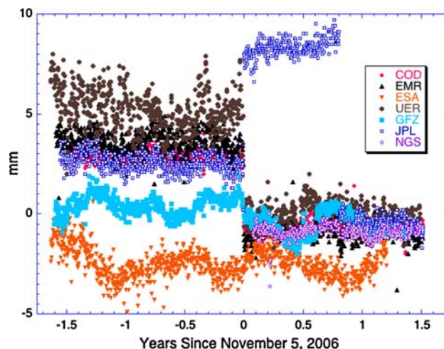
Fig. 7 The daily bias between ZPD product produced by each AC and the IGS ZPD product. For each day the bias is averaged over all sites and epochs
