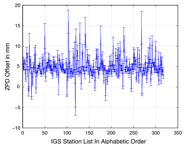
Fig. 11 The ZPD values from PCV case were subtracted from those of no-PCV case at matching time tags, and the daily mean values of ZPD differences are computed for each IGS ground station. Then, the mean and sigma of daily mean differences are computed for the period from November 11, 2007 to May 03, 2008. The x -axis denote the IGS ground stations in alphabetic order. The y -axis denote the mean and sigma value of the daily mean differences. A consistent bias between the two cases can be easily noted from this figure
