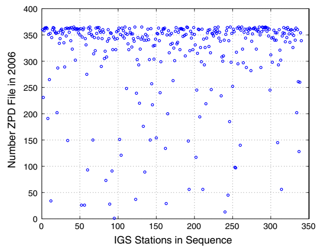
Fig. 6 The number of IGS troposphere ZPD files for each IGS ground station in year 2006
