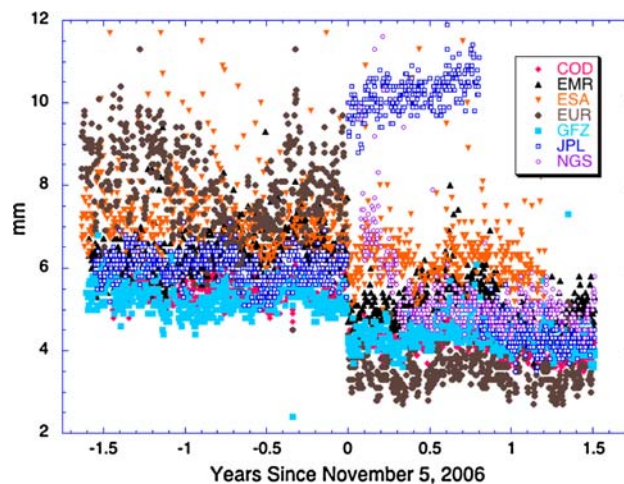
Fig. 8 The daily standard deviation for the ZPD product from each AC relative to the IGS ZPD product. For each day the standard deviation is computed from all sites epochs
