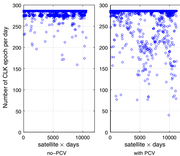
Fig. 9 The number of clock epochs in the IGS clock files for each satellite, during 1 year before November 2006 (no-PCV) and 1 year after November 2006 (with PCV). The x -axis denotes the satellite \times day ordinal number during the 1 year time span ( 365 \times 30 \approx 11000 ); Note the significantly increase in number of missing epochs after the transition to PCV modeling
