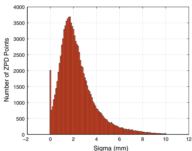
Fig. 2 Histogram of the formal errors reported for the legacy combined final troposphere solutions. The histogram was generated using 30 site solutions for year 2003. Zero sigma is reported when only one AC contributed a solution for a given site
