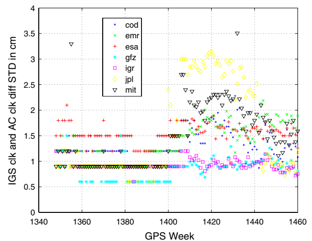
Fig. 10 The standard deviation value of difference between IGS combined clock solution and each AC's clock solution are extracted from IGS summary files from GPS week 1348 to 1460. This period spans 2 years with GPS week 1400 at the center. The x -axis denote the time in GPS week and the y -axis denote the standard deviation of clock difference in cm
