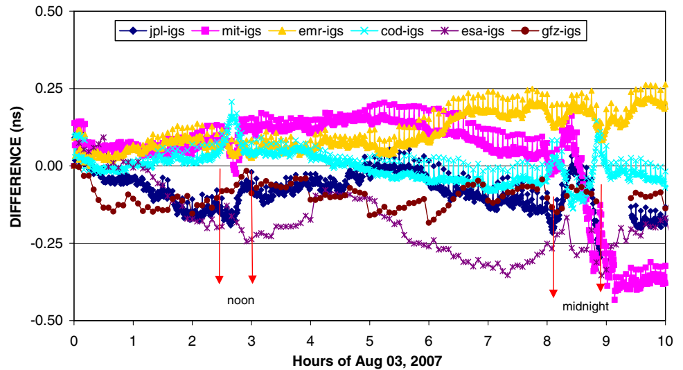
Fig. 1 AC PRN 5 clock differences during the noon and midnight turns ( |\beta| < 1.6^\circ ) on August 3, 2007. The problem of combination of 30-s and 5-min AC clocks caused the regular, 5-min spikes in the IGS 30-s clock combinations (this problem has been largely corrected in January 2008 (G. Gendt, personal communication))
