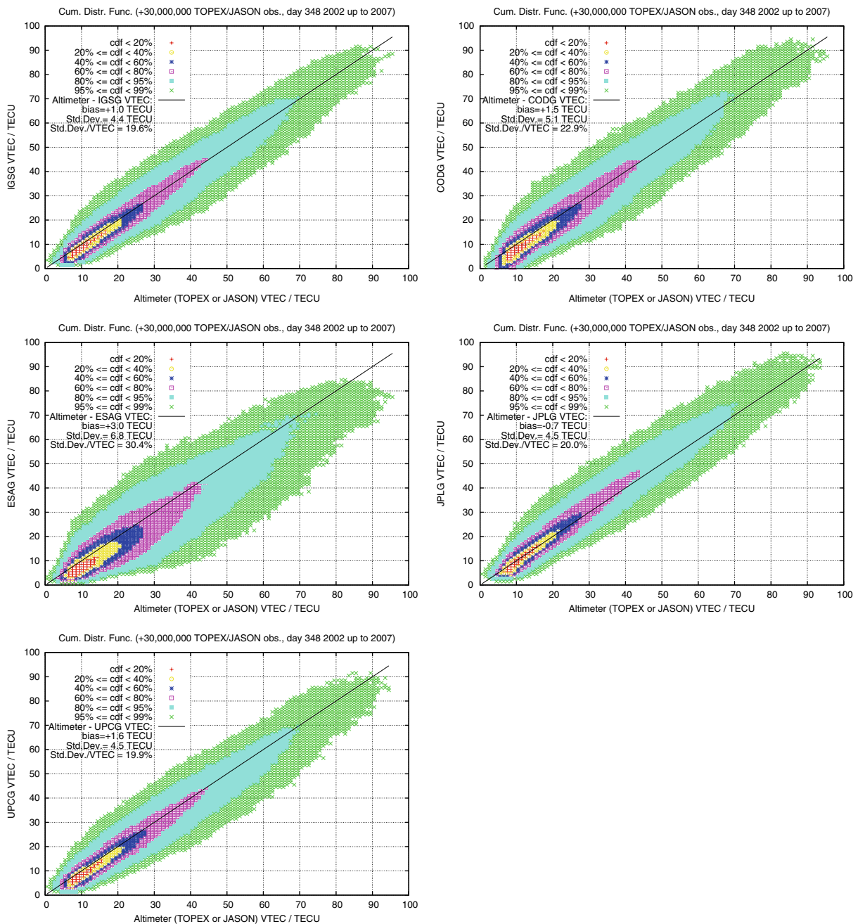
Fig. 14 Cumulative Distribution Function of VTEC discrepancy values provided by final VTEC maps (vertical axis) regarding to the VTEC values, directly observed by the TOPEX/JASON altimeters
