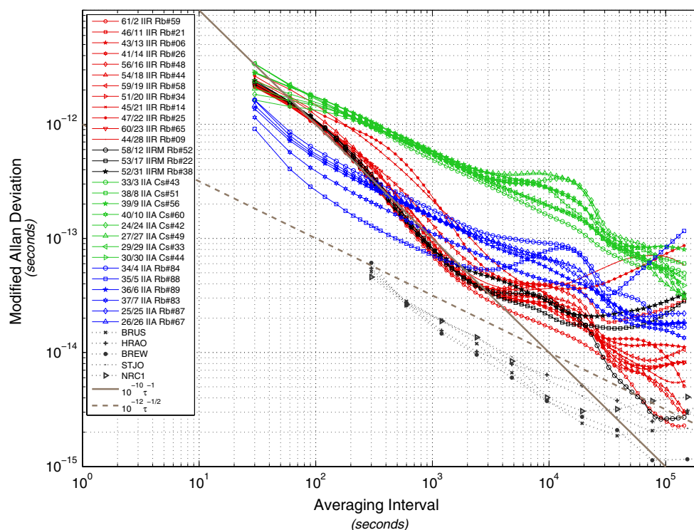
Fig. 1 Frequency instability (modified Allan deviation) of each GPS satellite and five ground stations for the period 15 June 2007 (MJD 54266) to 5 July 2007 (MJD 54286) using IGS Final clocks. The five ground clocks are among the highest-weighted clocks making up IGST during this period. All data were detrended by removing a second-order polynomial prior to calculating the MDEV. For satellites, the legend indicates the Navstar vehicle number/PRN code, satellite block, and the frequency standard type and serial number for the standard active during this period. For reference, lines varying as \tau^{-1} , flicker phase, and \tau^{-1/2} , random walk phase, are drawn
