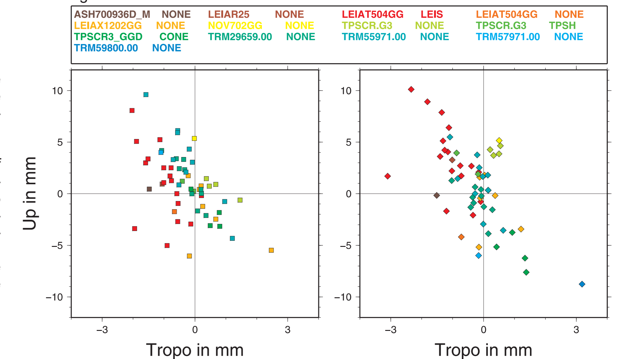
Figure 5: The mean GPS/GLONASS biases for all stations with ROBOT specifically calibrated antennas for GLONASS are plotted. In nearly all cases the differences between the squares (IGS05-based solution) and diamonds (IGS08-based solution) are on the 2 to 3 mm level for the vertical component. Only a few stations show a significant difference, like DARW and YAR3. In the horizontal components both sets of GPS/GLONASS biases agree on the one-mm level.
