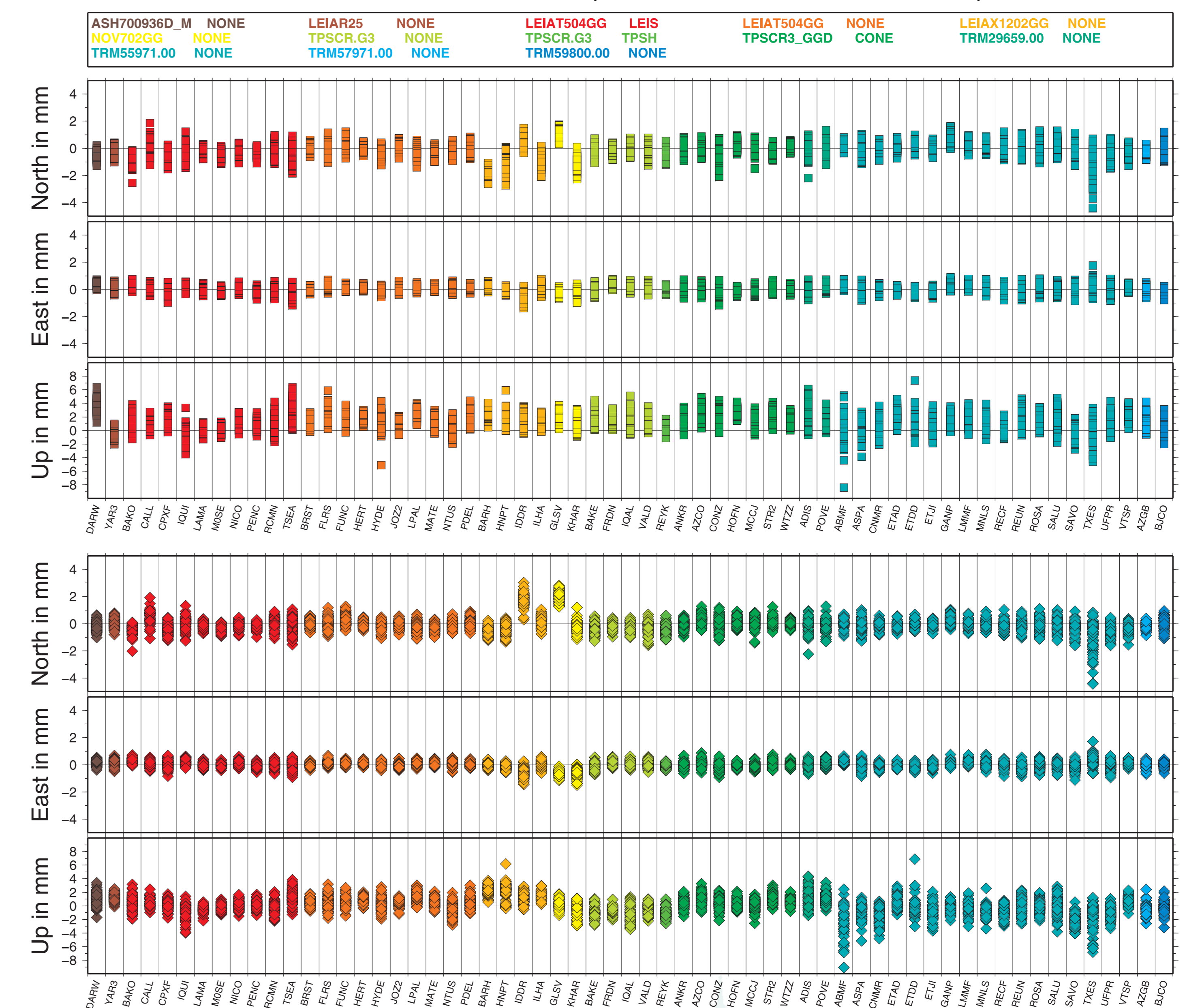
Figure 7: Differences in the computed weekly station coordinates between the default and the solution with the GPS/GLONASS bias estimation. In the top plot the IGS05-based and in the bottom plot the IGS08-based solution is presented. It is noticeable that all differences in the IGS05-based solution have a positive sign in the vertical component. This may be explained by a GLONASS-related scale inconsistency, e.g., due to the satellite antenna offsets. In the IGS08-based solution this feature is not visible. Nevertheless, there are systematic effects in the vertical component as well, e.g., most of the TRIMBLE-antennas show negative differences but in the results for stations equipped with LEICA- or TOPCON-antennas positive signs dominate.
