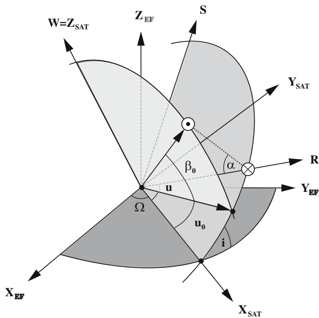
Fig. 1 Elevation of the Sun with respect to the orbital plane: Earth-fixed system ( X_{EF} , Y_{EF} , Z_{EF} ), orbit system ( X_{SAT} , Y_{SAT} , Z_{SAT} ), satellite system ( R , S , W ). Right ascension of the ascending node \Omega , argument of latitude u , inclination i , argument of latitude u_0 and elevation \beta_0 of the Sun. \odot symbolizes the Sun, \otimes the satellite
