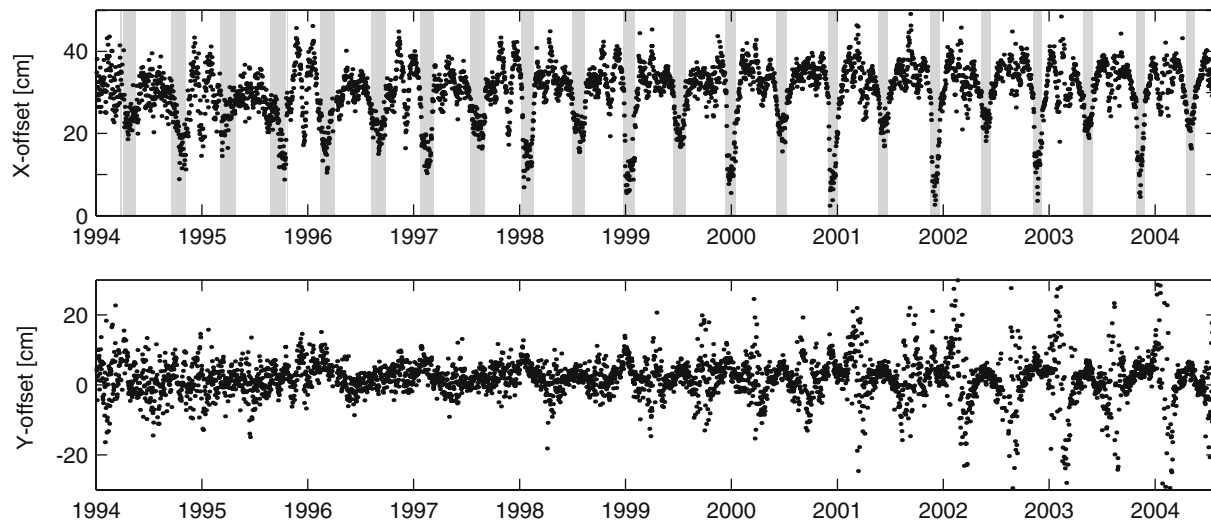
Fig. 5 Horizontal offset time series for SVN 37 (PRN 07). The eclipse seasons are gray-shaded . The maximum elevation of the Sun above the orbital plane \beta_{0,\max} steadily increases after 1996.
