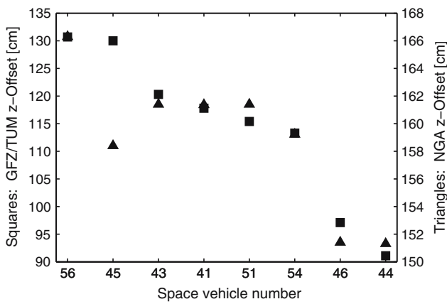
Fig. 13 Comparison of individual antenna z-offsets (cm) for all Block IIR-A satellites: the GFZ/TUM offsets are represented by squares with the scale on the left, whereas the scale for the triangles representing the NGA values is given on the right
