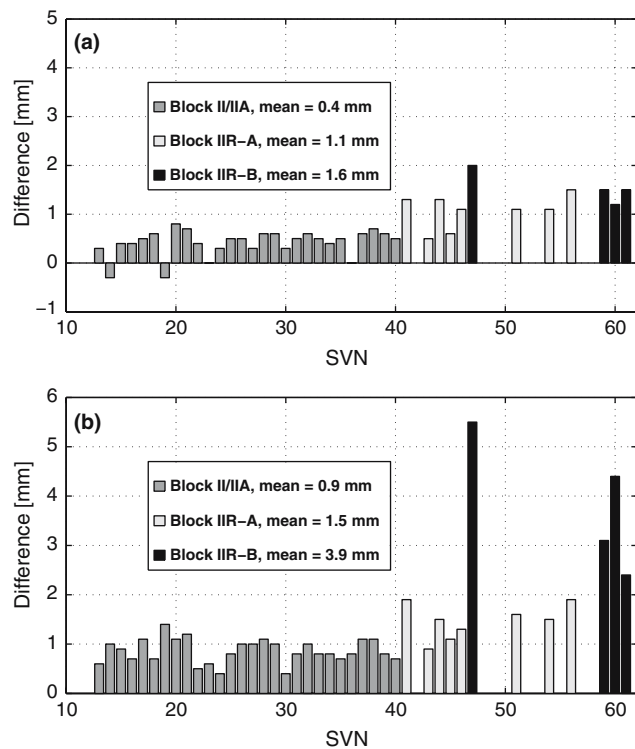
Fig. 16 RMS reduction of 3-day orbit fits through three 1-day orbital arcs: a relative PCVs (solution A) versus absolute PCVs with block-specific z -offsets (solution B), b relative PCVs (solution A) versus absolute PCVs with satellite-specific z -offsets (solution D). Due to their small number of observations, Block I satellites were excluded
