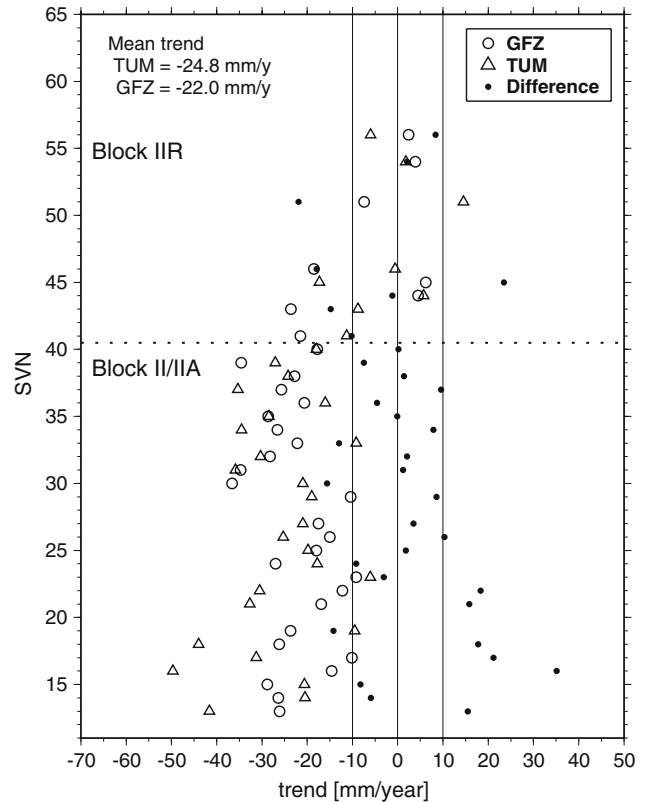
Fig. 11 Trends for satellite antenna z-offsets for individual satellites from GFZ and TUM using own PCVs and fixing the reference frame to IGB00. Only satellites with more than 2 years of data are shown. The formal trend error is in the range of 2–5 mm/year
