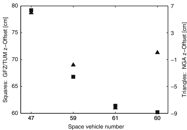
Fig. 14 Comparison of individual antenna z-offsets (cm) for all Block IIR-B satellites: the GFZ/TUM offsets are represented by squares with the scale on the left, whereas the scale for the triangles representing the NGA values is given on the right
