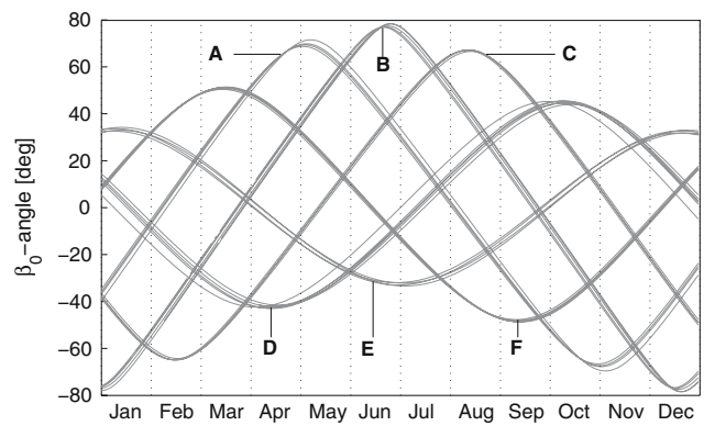
Fig. 2 Elevation of the Sun \beta_0 with respect to the orbital planes (A–F) for all GPS satellites in 2003
