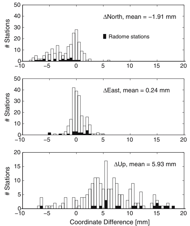
Fig. 17 Histograms of the mean coordinate changes between the solutions with relative (solution A) and absolute PCVs (solution D). Geocenter differences were removed by a three-parameter similarity transformation
